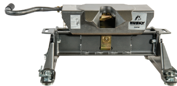
GM®/Chevy® Upright Shown
